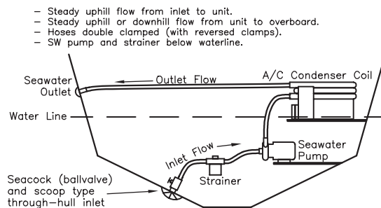
Figure 1: Typical Seawater Plumbing System
