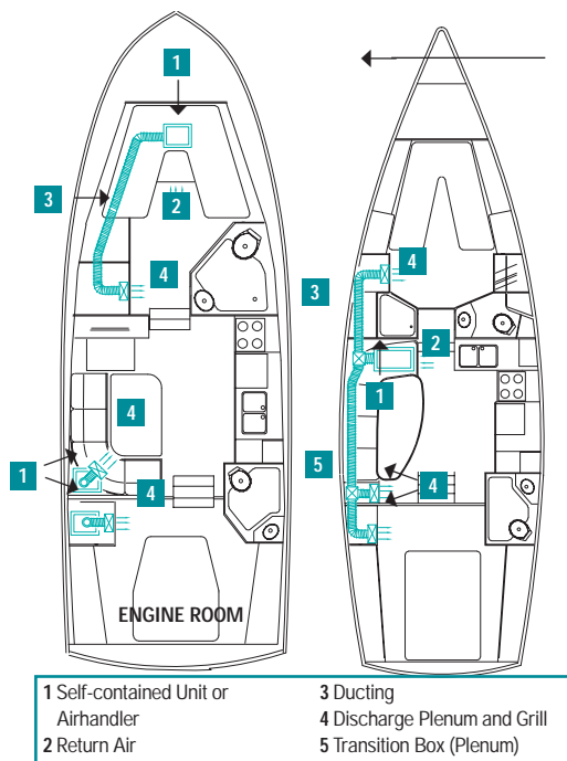
Figure 3: Comparison of typical central and self-contained systems
